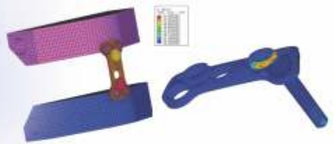
CerviEdge Finite Element Analysis to test fatigue life performance of implant construct
